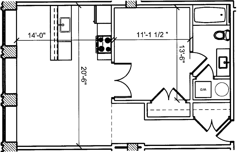
UNIT TYPE 04 ONE BEDROOM
