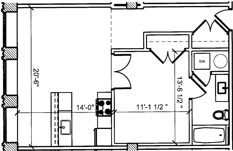
UNIT TYPE 01 ONE BEDROOM
